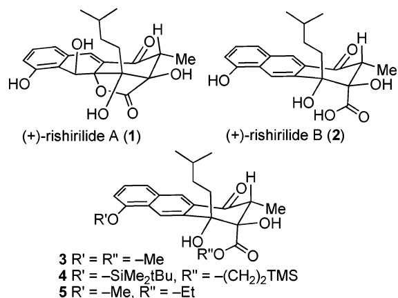
Figure 1. The natural products (+)-rishirilides A ( 1 ) and B ( 2 ), and some known derivatives ( \pm )- 3 , ( \pm )- 4 , and ( \pm )- 5 .
