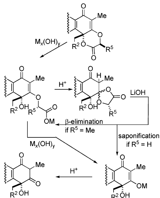
Figure 3. Lactate and glycolate derivatives behave differently.
