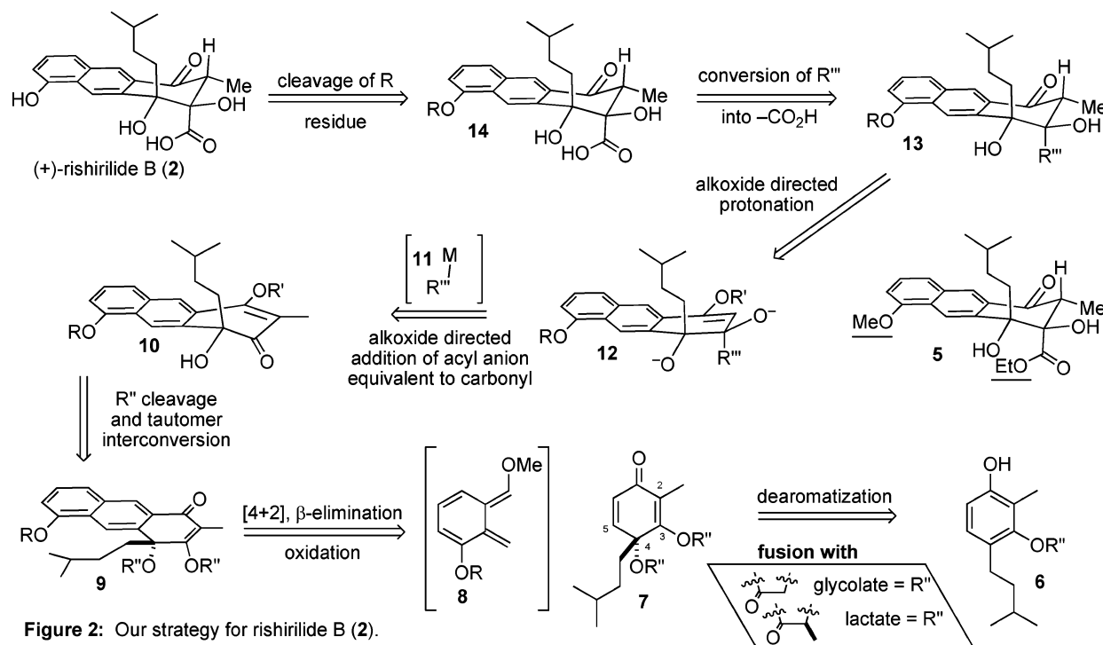
Figure 2. Our strategy for rishirilide B (2).
