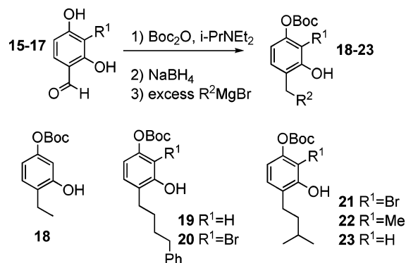
Scheme 1. Synthesis of Differentially Protected 4-Alkyl Resorcinols
